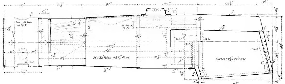
Boiler for Lehigh Valley Pacific Type Locomotives
